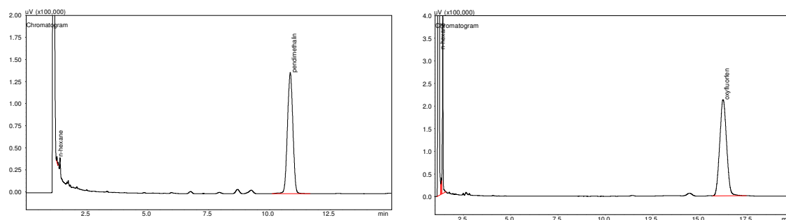
Fig.1: Standard chromatograms of pendimethalin and oxyfluorfen (1 µg ml -1 )
