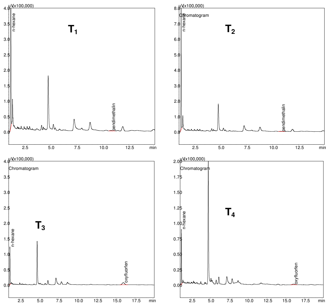
Fig.4: Chromatograms showing pendimethalin (0.5 (T 1 ) and 0.75(T 2 ) kg a.i ha -1 ) and oxyfluorfen (0.1(T 3 ) and 0.15(T 4 ) kg a.i. ha -1 ) residues in raddish tubers
