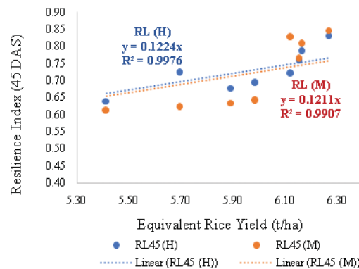
Fig. 5: Relationship between Resilience Index and Equivalent rice yield of soil under CA based R-W system RS, Resistance index; H, Heat stress; M, Moisture stress
